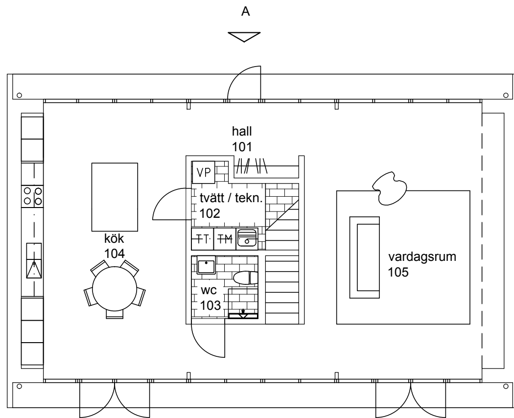
bottenplan
