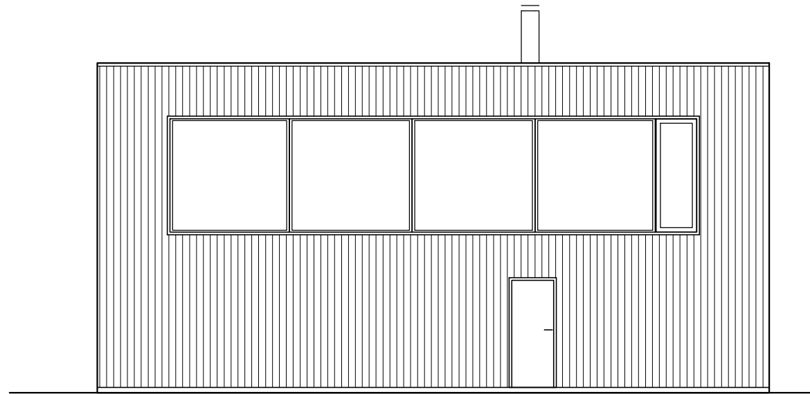
fasad A
