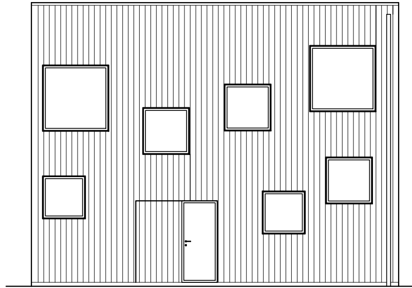
fasad A
