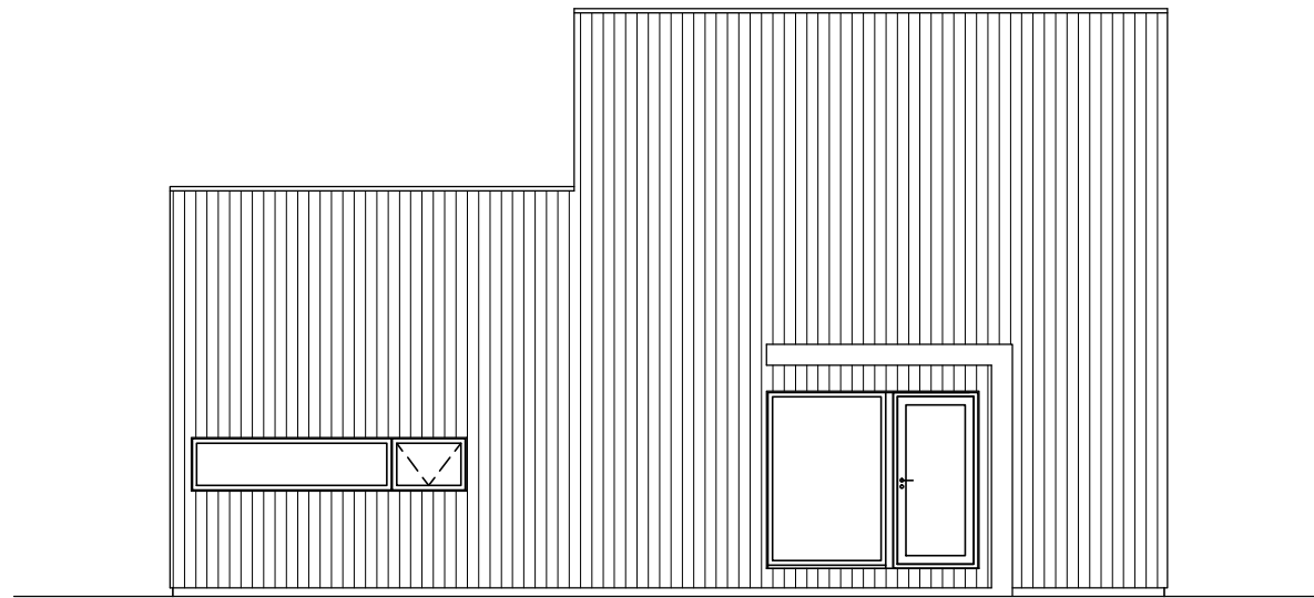
fasad A
